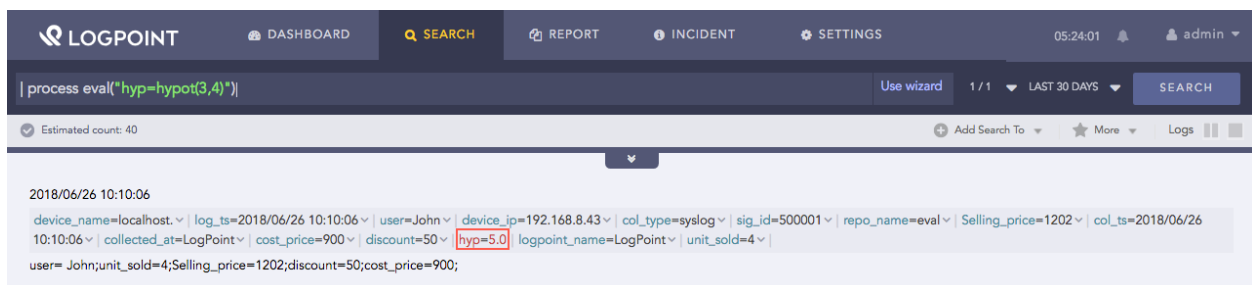
Fig. 13: Hypot function
