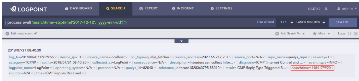
Fig. 5: Strptime function
