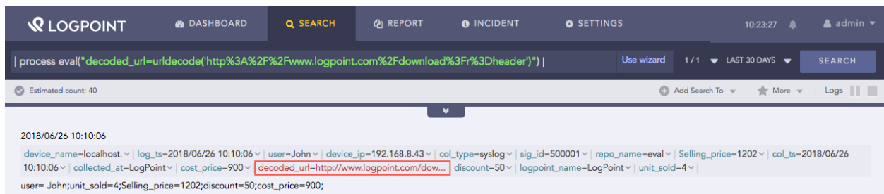
Fig. 10: Urldecode function
