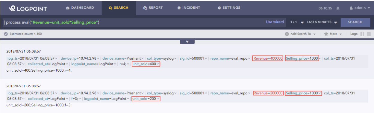
Fig. 1: Eval Expression
