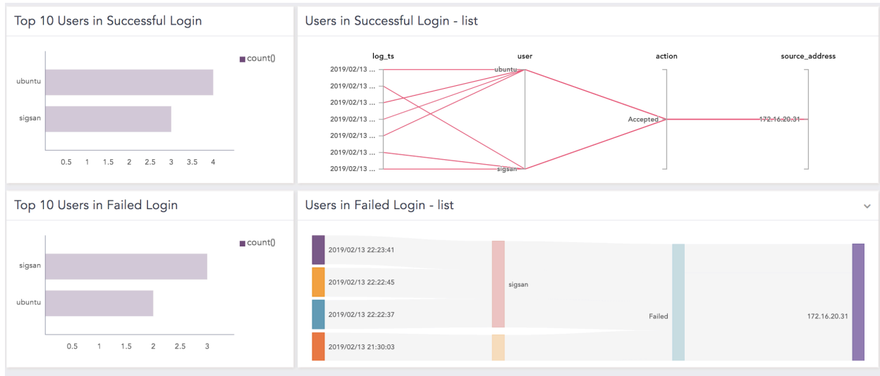
Fig. 4: Unix Dashboard
